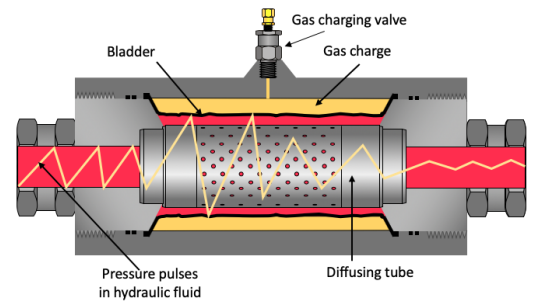
Noise Suppressor
