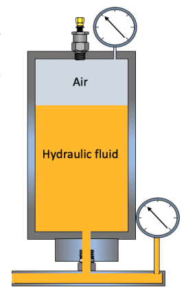
Air-Over-Oil Accumulator
