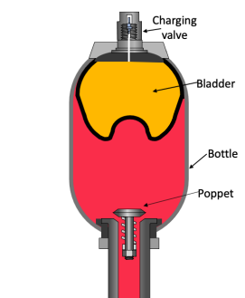
Bladder Accumulator, Fully-Charged
