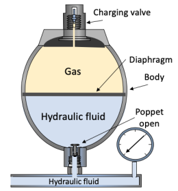
Diaphragm Accumulator Before Pre-Charge
