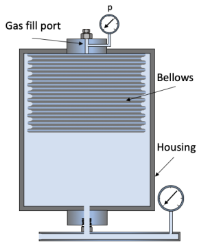
Bellows Accumulator Before Any Gas or Hydraulic Pressure
